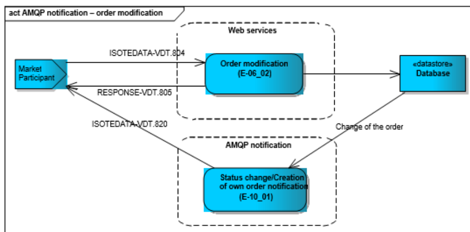
Figure 42 Sending messages scheme – order modification (AMQP notification)
