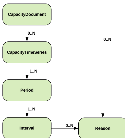
Figure 51 Schema of CapacityDocument structure
