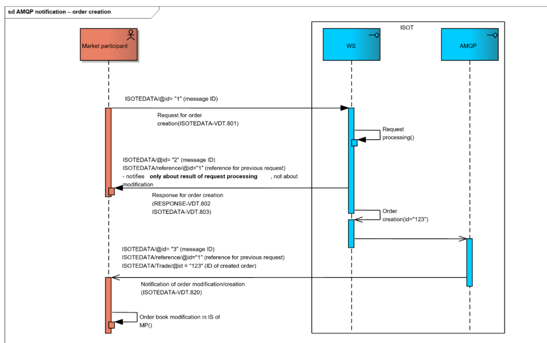
Figure 41 Order of send messages scheme – order creation (AMQP notification)
