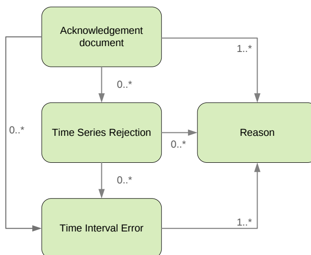
Figure 50 Scheme of Acknowledgement structure
