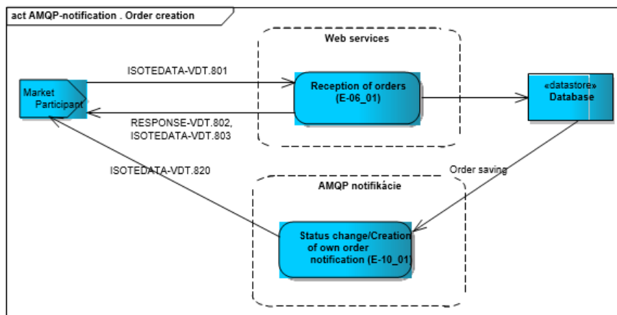
Figure 40 Sending messages scheme – order creation (AMQP notification)
