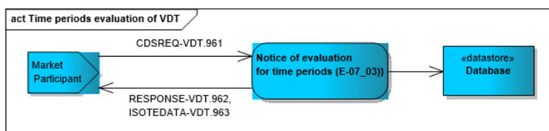
Figure 39 Notice of an evaluation for time periods scheme
