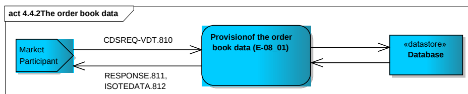
Figure 28 Provision of order book data scheme
