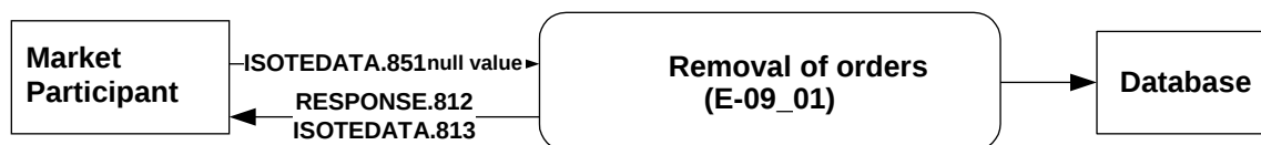
Figure 31 Schema for IDA order removal
