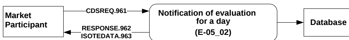
Figure 36 Notification schema of evaluations for day for market participant
