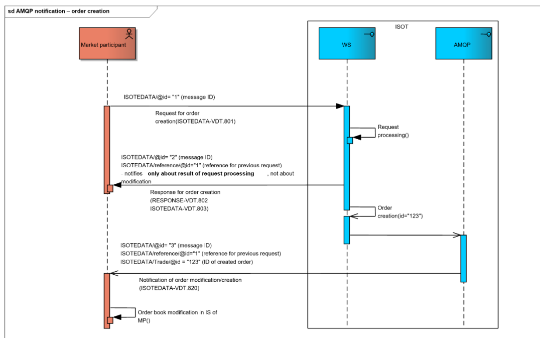
Figure 40 Order of sended messages scheme – order creation (AMQP notification)
