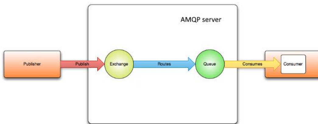
Figure 9 AMQP communication concept
