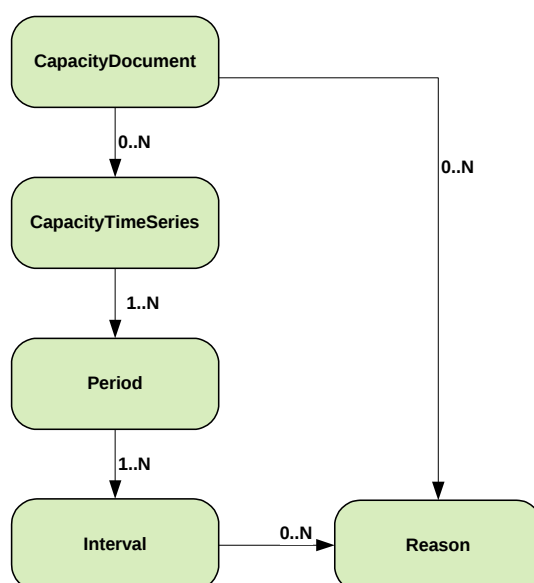
Figure 50 Schema of CapacityDocument structure
