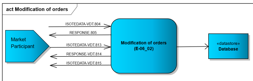
Figure 25 Reception of order scheme
