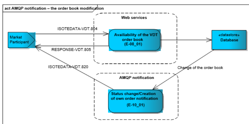
Figure 43 Sent messages scheme – order creation (AMQP notification)
