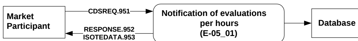
Figure 34 Notification schema of evaluations per hours for market participant
