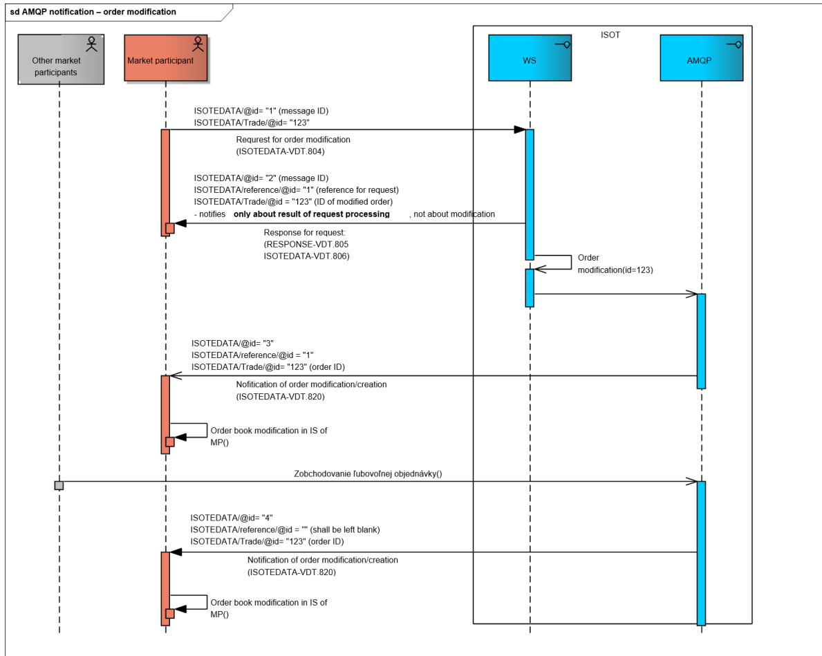
Figure 42 Order of sent messages scheme – order modification (AMQP notification)
