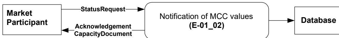
Figure 48 Notification schema of MCC values
